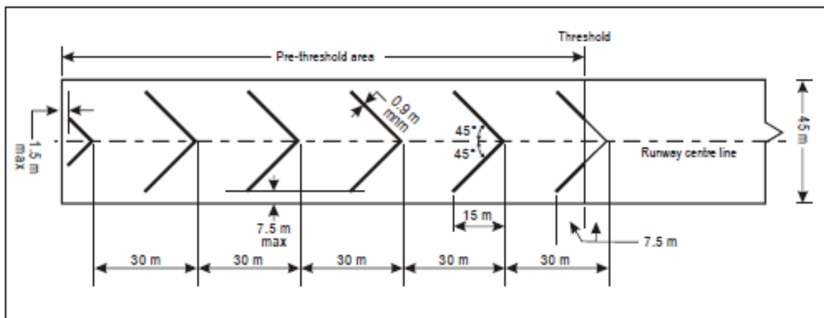
Figure 10-2. Pre-threshold marking
