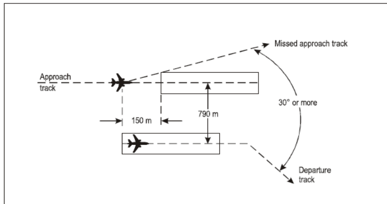
Figure 6-39. Segregated parallel operations where runways are staggered (see 6.7.3.56.2)
