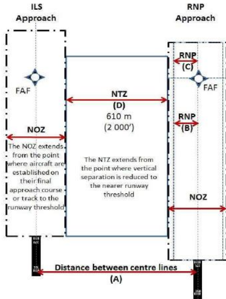
Figure 6-1 Distance between centre lines, NTZ and NOZ.
