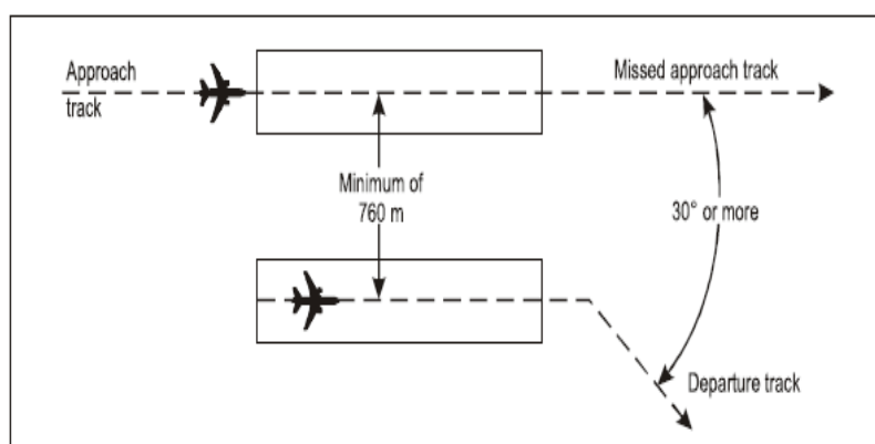
Figure 6-17. Segregated parallel operations (see 6.7.3.56.1 b))
