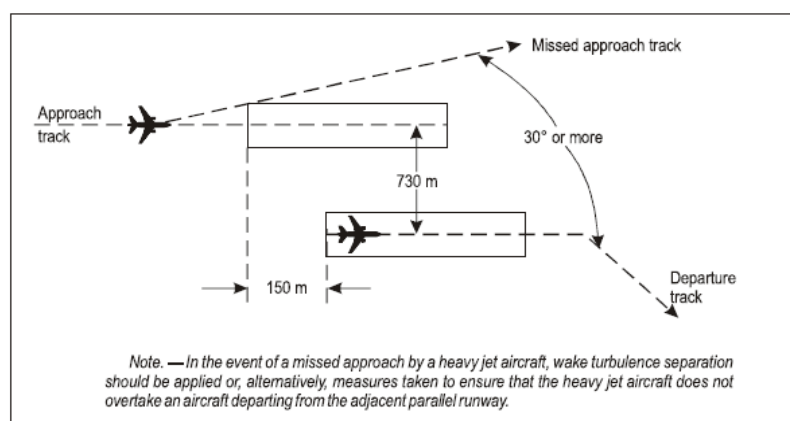
Figure 6-28. Segregated parallel operations where runways are staggered (see 6.7.3.56.2)
