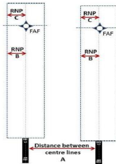
Figure 6-2— RNP value and distance between centre lines
