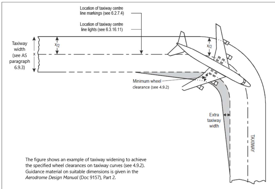
Figure 4-1. Taxiway curve
