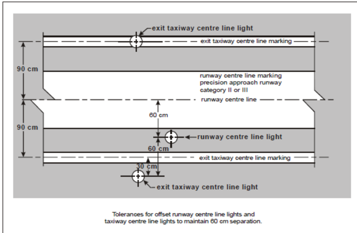
Figure 6-5. Offset runway and taxiway centre line lights
